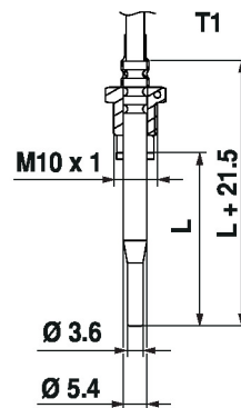
T1: Temperatursensor
